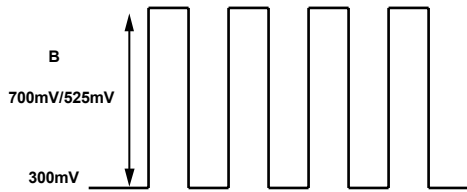
Figure 124. SD/ED RGB Output Levels—RGB Sync Disabled
