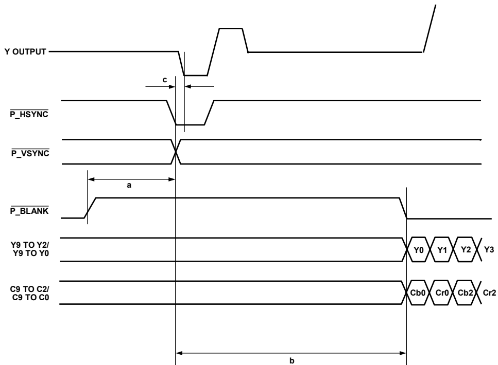
Figure 15. ED-DDR, 8-/10-Bit, 4:2:2 YCrCb ( \overline{\text{HSYNC}} / \overline{\text{VSYNC}} ) Input Timing Diagram
