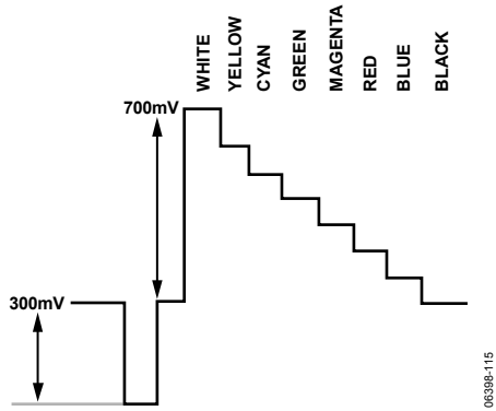
Figure 114. Y Levels—NTSC
