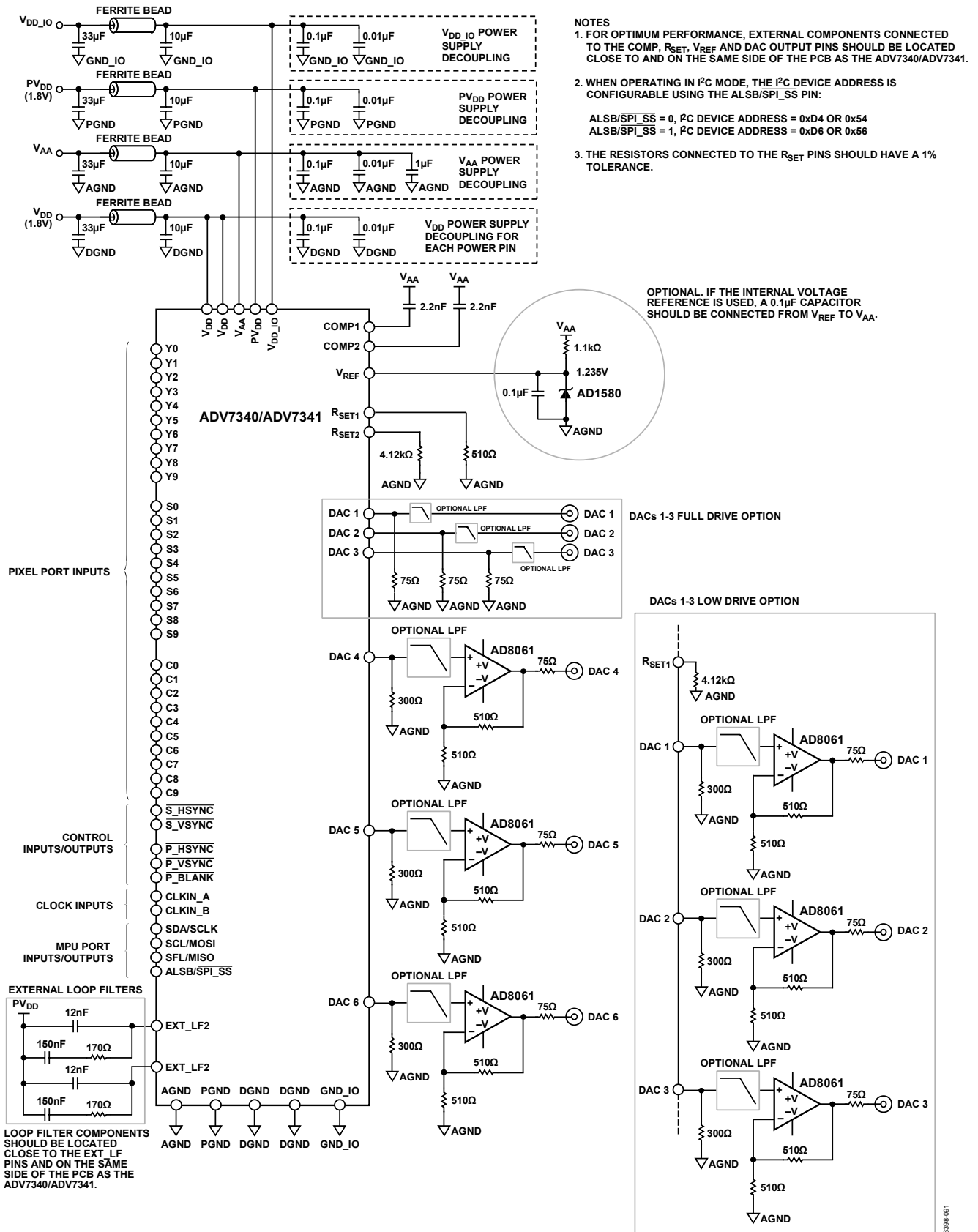
Figure 90. ADV7340/ADV7341 Typical Application Circuit
