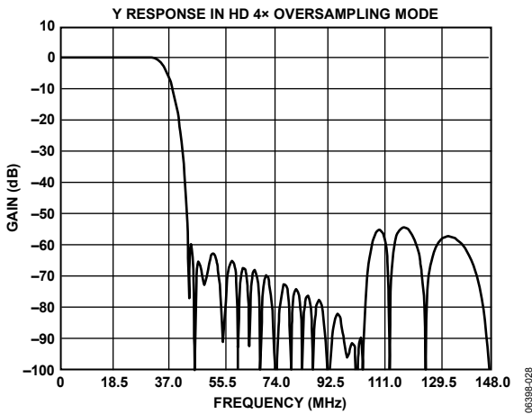
Figure 28. HD 4x Oversampling, Y Filter Response
