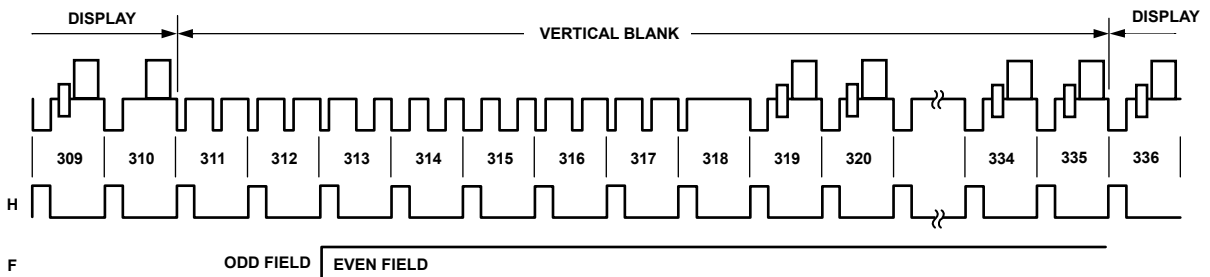
Figure 102. SD Master Mode 0, PAL
