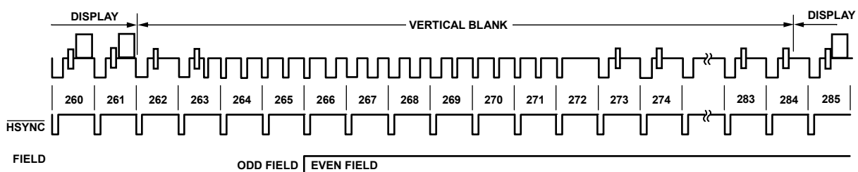
Figure 104. SD Slave Mode 1, NTSC
