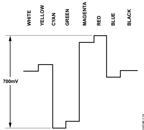
Figure 118. Pr Levels—PAL
