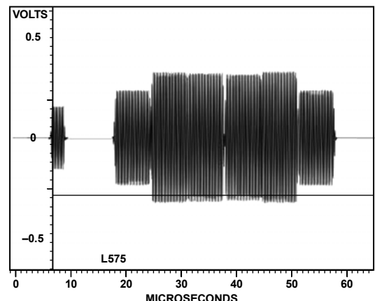
Figure 132. PAL Luma
