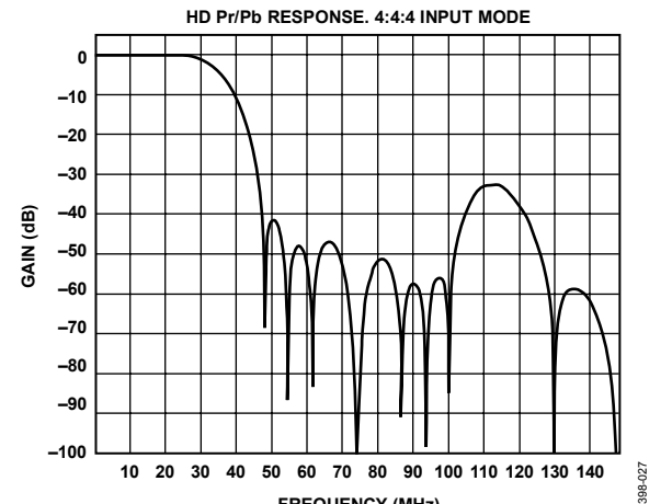
Figure 27. HD 4x Oversampling, PrPb (SSAF) Filter Response (4:4:4 Input)
