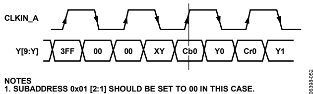
Figure 52. ED/HD-DDR Input Sequence (EAV/SAV)—Option A
