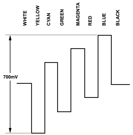
Figure 119. Pb Levels—PAL
