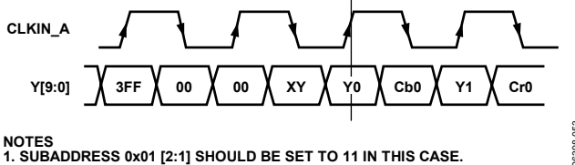
Figure 53. ED/HD-DDR Input Sequence (EAV/SAV)—Option B
