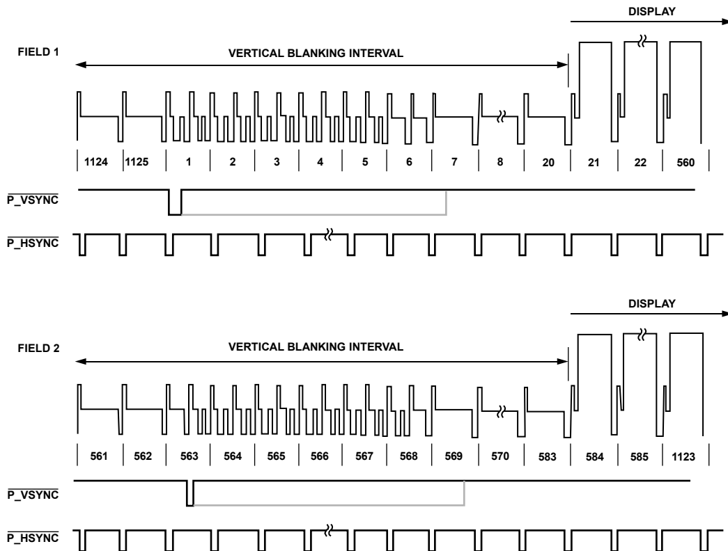
Figure 113. 1080i \overline{HSYNC} and \overline{VSYNC} Input Timing
