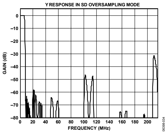
Figure 34. SD, 16x Oversampling, Y Filter Response
