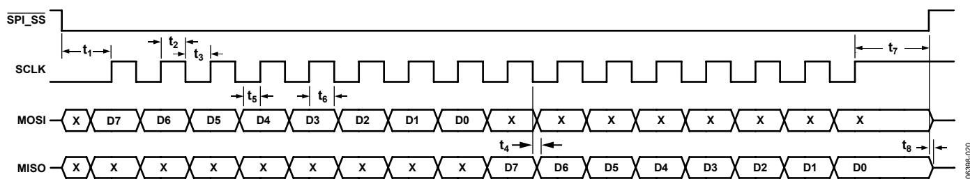
Figure 20. MPU Port Timing Diagram (SPI Mode)
